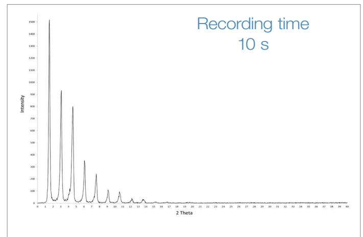
Silver Behenate powder sample recorded on ARL EQUINOX 100 in reflection mode.
